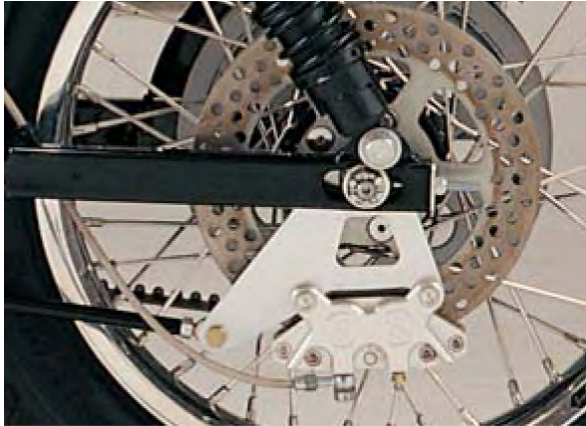
10" Rear Disc Brake Kit
